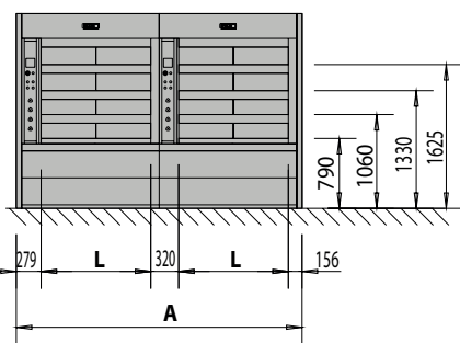
Mod. 124+124 - 4 Chambers
