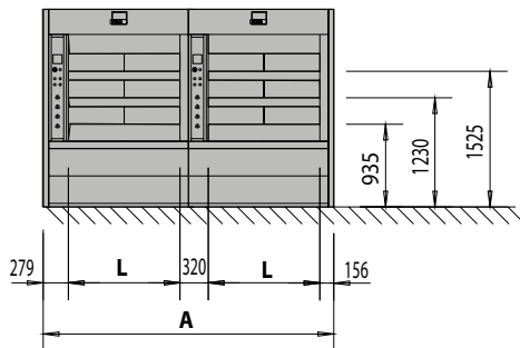
Mod. 124+124 - 3 Chambers
