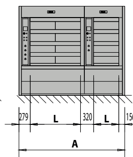
Mod. 62+124 - 3 Chambers
